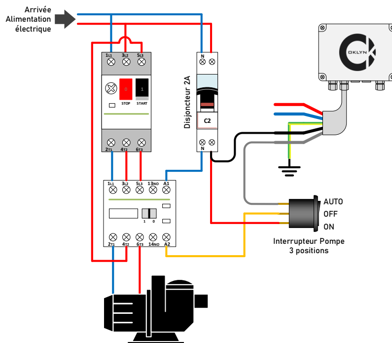
Figure 13 : Raccordement commande pompe (nouvelle installation)
