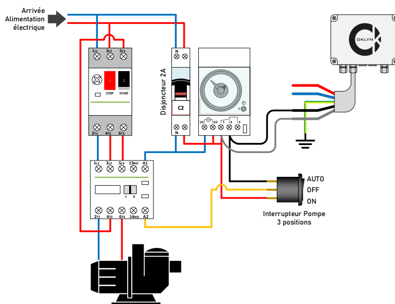
Figure 14 : Raccordement commande pompe (installation existante)
